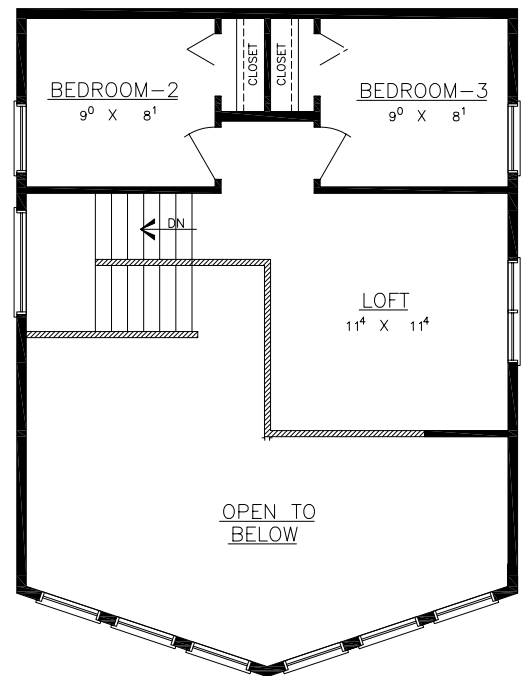
SECOND FLOOR AREA = 366 S.F.
